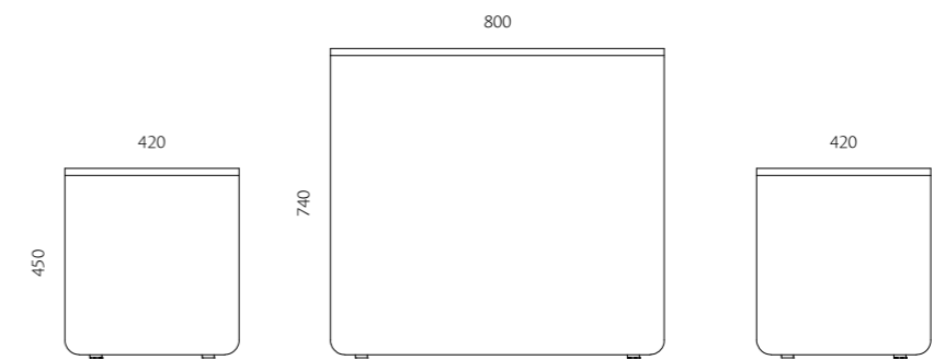
Campus table and bench
